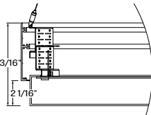
PCSQPD1 + 2D - 2" drop lens
