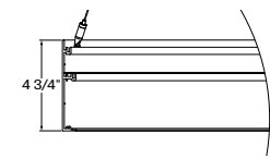
PCSQPD1 + FH - Flush lens
