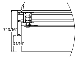
PCSQPD1 + 3D - 3" drop lens
