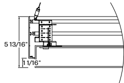
PCSQPD1 + 1D - 1" drop lens
