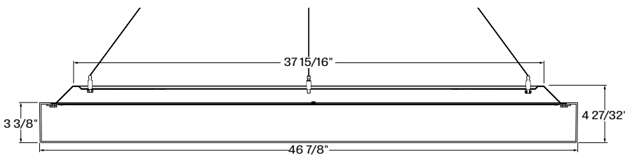
POROPD + 3H - Pop Round Pendant with 3.5" optic
